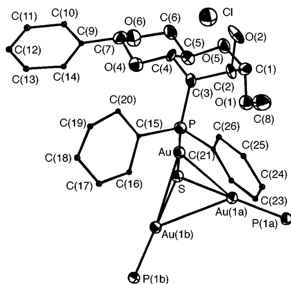
Fig. 3 Partial view of compound 2 with the atom labelling of the chiral phosphine ligand
