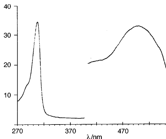
Fig. 5 Uncorrected solid-state excitation and emission spectra for the complex [\{\text{Au}(\text{mbpa})\}_3\text{S}]\text{Cl} 2 at room temperature
