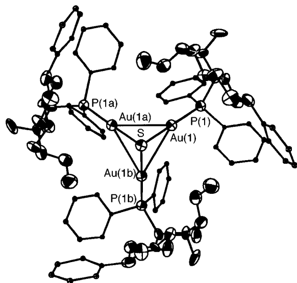
Fig. 2 Structure of the cation [Au(mbp)_3]_3S]^+ of complex 2 . Hydrogen atoms are omitted for clarity.
